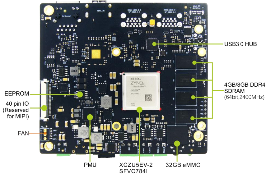
FZ5 Card Top-View (delivered with active heatsink by default)
